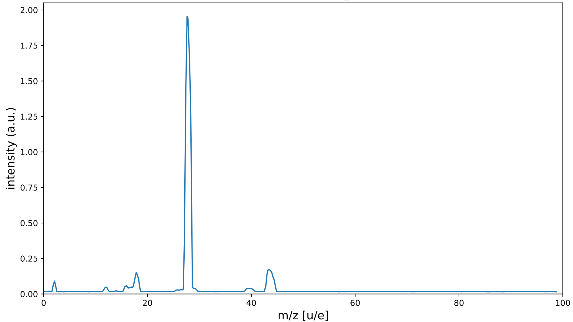
QMS-TPD: residual gas_8.txt
